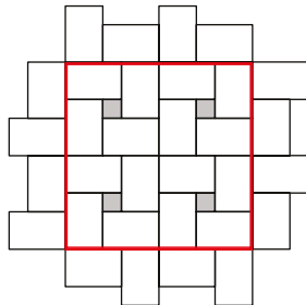
VM-16 30x20 (16 db/m 2 ), 10x10 (4 db/m 2 )
