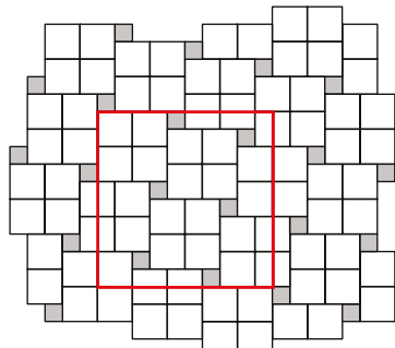
VM-15 20x20 (23,5 db/m 2 ); 10x10 (6 db/m 2 )
