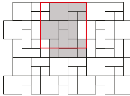
VM-25 40x40; 40x20; 20x20 (2; 6; 4 db/m 2 )
